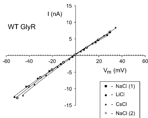
FIGURE 5 Examples of whole cell I/V curves for the WT GlyR channel. The measurements were all made in the same cell in external solutions of control NaCl [NaCl(1)], then sequentially LiCl, CsCl, and finally back to NaCl [NaCl(2)], as indicated in the inset legend. Throughout each experiment, the NaCl composition of the cell was not changed. The V_m values were corrected for liquid junction potentials in each case. The aim was to measure the slope conductance at -40 mV for each solution (see Table 3 for averaged values), which should include a component of the conductance due to the cation counterions, anticipated at that potential to have a major contribution from the counterions in the external solution (see text). It may be seen that there is a small reduction in the slope conductance at -40 mV going from the external NaCl solution to the external LiCl solution and a small increase in slope conductance going to the external CsCl solution (see Table 3 for averaged values). The aim was to compare this relative shift in conductance with the prediction that the \text{Cl}^- conductance component was not dependent on the counterion.
