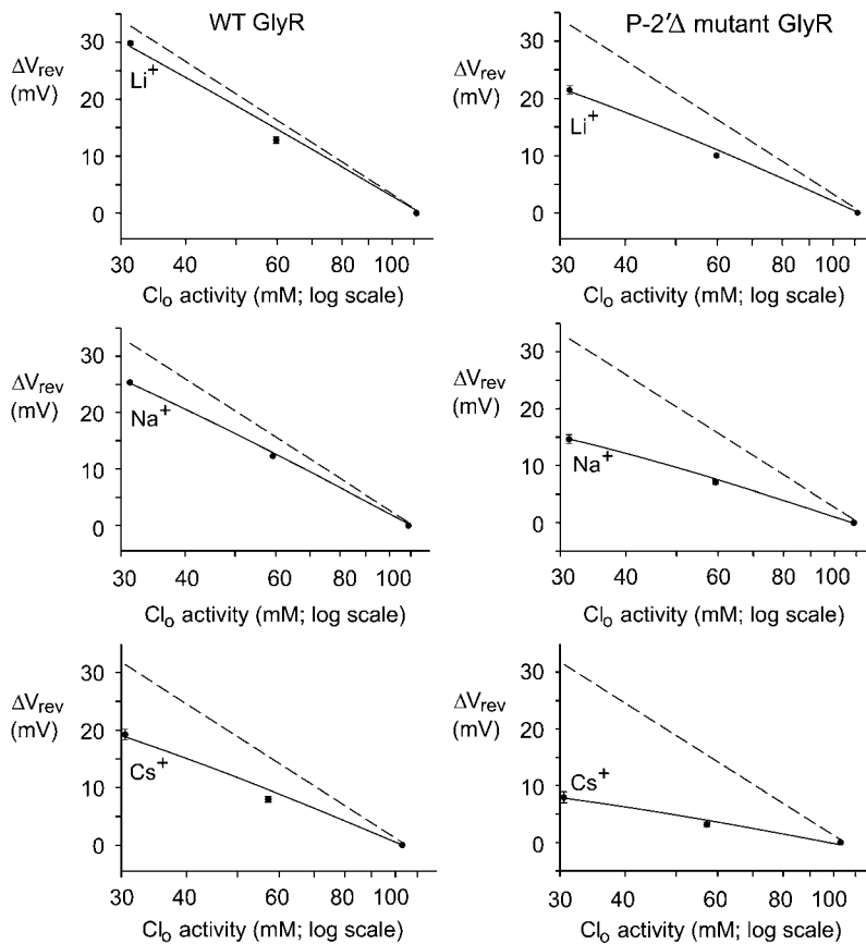
FIGURE 3 Semilogarithmic plots of the average shifts in reversal potential, \Delta V_{rev} , versus external \text{Cl}^- activity (on a log scale) for the anion-selective WT and P-2' \Delta GlyR channels in 1, 0.5 and 0.25 LiCl, NaCl, and CsCl solutions. The solid lines show fits of the GHK equation (Eq. 2) to the \Delta V_{rev} values, as used to determine P_{\text{Cl}}/P_{\text{Na}} averaged from individual experiments and shown in Figs. 1 and 2. The dashed lines indicate the \Delta V_{rev} values expected if the counterion permeability had been zero. The errors shown, when larger than symbols, are the SEs.
