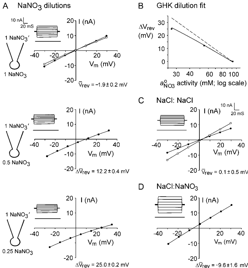
FIGURE 4 Dilution potentials in \text{NaNO}_3 solutions and biionic \text{NaCl}:\text{NaNO}_3 solutions to determine relative P_{\text{NO}_3}/P_{\text{Na}} and P_{\text{NO}_3}/P_{\text{Cl}} values, respectively, for the WT \alpha 1 GlyR channel. (A) Sample whole cell measurements of I/V curves in different dilutions of \text{NaNO}_3 solutions to determine P_{\text{NO}_3}/P_{\text{Na}} . The experimental procedures are identical to those described for Fig. 1 and the solution composition is given in Materials and Methods. As in Figs. 1 and 2, the \Delta V_{\text{rev}} values for the 0.5 and 0.25 dilution solutions are both positive, indicating that the WT GlyR channel is still anion-selective when \text{NO}_3^- replaces \text{Cl}^- . (B) Semilogarithmic plots of the averaged shifts in reversal potential versus external \text{NO}_3^- activity (on a log scale). The solid lines show the fits of the GHK equation (Eq. 3) to these \Delta V_{\text{rev}} values, as used to determine P_{\text{NO}_3}/P_{\text{Na}} , averaged from individual experiments and shown in panel A. Again, as in Fig. 3, the dashed line indicates the \Delta V_{\text{rev}} values expected if the counterion permeability had been zero. (C and D) Sample I/V curves in symmetrical \text{NaCl} solutions (C), before (solid circles) and after (open circles) measurements of biionic potentials in \text{NaCl}:\text{NaNO}_3 solutions (D). Both panels A and B are for the same cell, and panels C and D are for the same cell (though for a different one from that in panels A and B). The insets with the I/V curves show representative current traces in response to voltage steps (from 0 mV to -30 mV) (lower traces) through to +30 mV (top traces) in increments of 10 mV. The lower sets of current traces in each panel show control responses in the absence of glycine.
